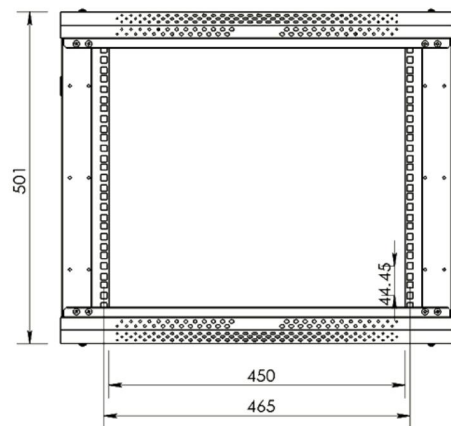
Inside view
